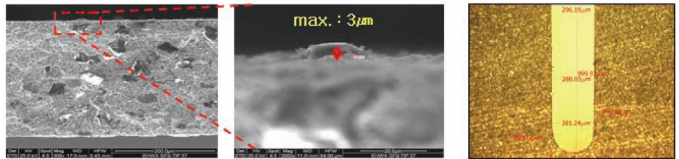
[New Blade Surface and edge shape deformation]
