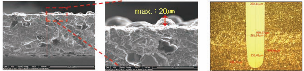
[Conventional Blade Surface and edge shape deformation]
